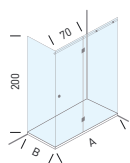
Hinged door and fixed short side glass panel (corner version)
