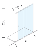
SLIDING DOOR AND FIXED GLASS PANEL recessed version
