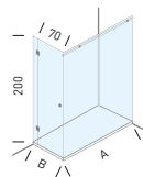
Hinged door and fixed long side glass panel (corner version)
