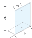
Hinged door and fixed glass panel (recessed version)
